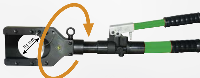
Prod.-No. 04015 head can be rotated through 320°
