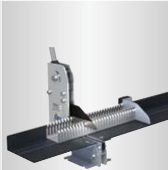
Wiring duct cutting device
